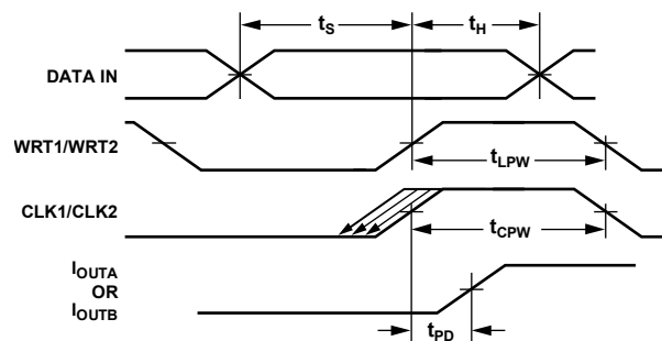
Figure 62. Dual-Port Mode Timing
