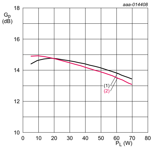
V_{DS} = 28\text{ V} ; I_{Dq} = 330\text{ mA} (main device); V_{GS(amp)peak} = 0.55\text{ V} . (1) f = 2496\text{ MHz} (2) f = 2690\text{ MHz}
