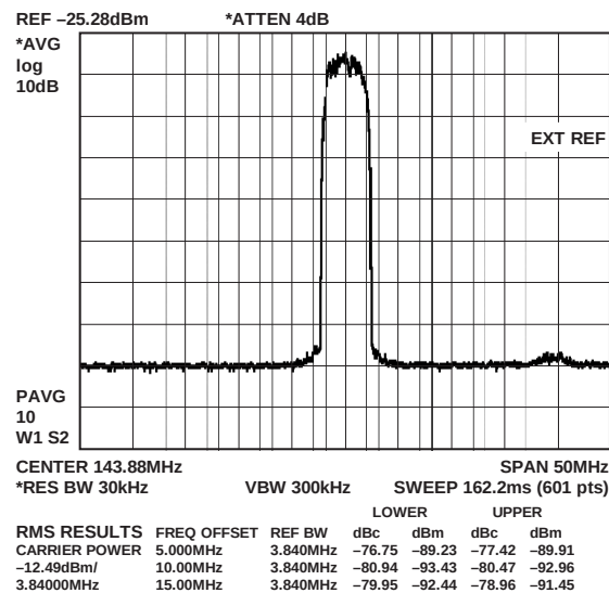
Figure 32. AD9779A W-CDMA Signal, 4× Interpolation, f_{DATA} = 122.88 MSPS, f_{DAC}/4 Modulation
