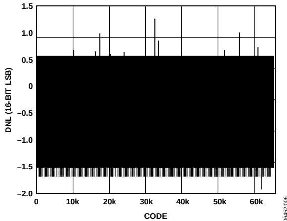
Figure 7. AD9779A Typical DNL
