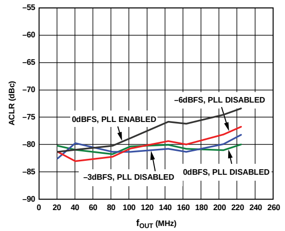
Figure 34. AD9779A ACLR for Third Adjacent Band W-CDMA, 4× Interpolation, f_{DATA} = 122.88 MSPS, On-Chip Modulation Translates Baseband Signal to IF
