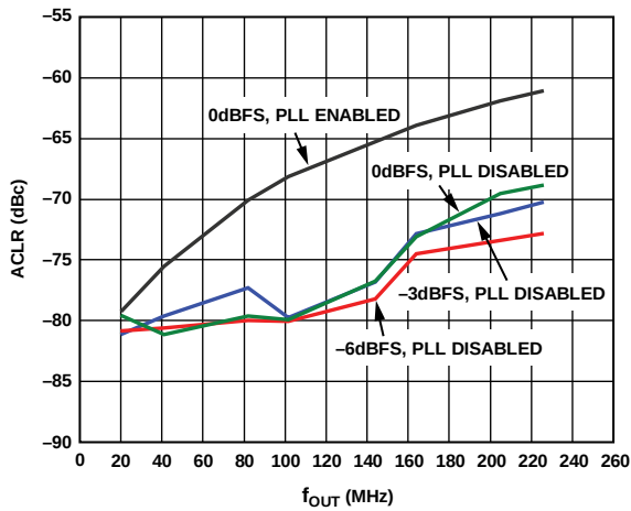
Figure 31. AD9779A ACLR for First Adjacent Band W-CDMA, 4× Interpolation, f_{DATA} = 122.88 MSPS, On-Chip Modulation Translates Baseband Signal to IF
