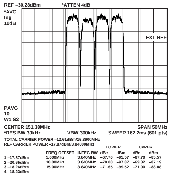
Figure 35. AD9779A Multicarrier W-CDMA Signal, 4× Interpolation, f_{DAC} = 122.88 MSPS, f_{DAC}/4 Modulation
