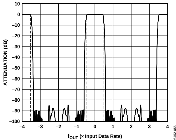
Figure 58. 4× Interpolation, Low-Pass Response to \pm 4\times Input Data Rate (Dotted Lines Indicate 1 dB Roll-Off)
