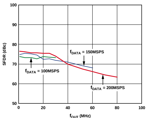
Figure 13. AD9779A Out-of-Band SFDR vs. f_{OUT} , 4 \times Interpolation
