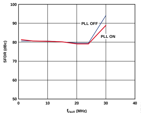
Figure 15. AD9779A In-Band SFDR vs. f_{OUT} , 4 \times Interpolation, f_{DATA} = 100 MSPS, PLL On/Off
