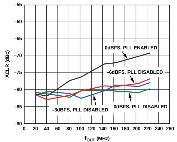
Figure 33. AD9779A ACLR for Second Adjacent Band W-CDMA, 4× Interpolation, f_{DATA} = 122.88 MSPS, On-Chip Modulation Translates Baseband Signal to IF
