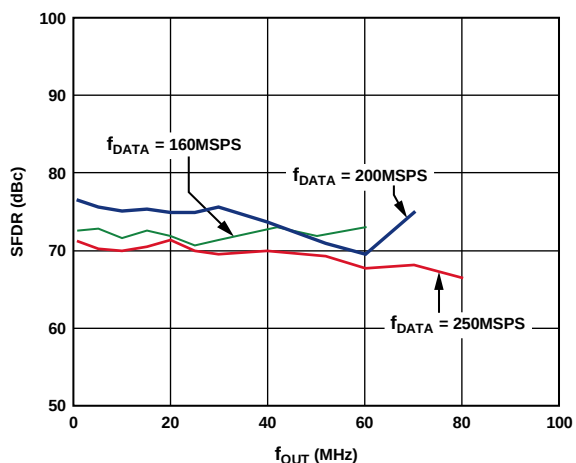
Figure 12. AD9779A Out-of-Band SFDR vs. f_{OUT} , 2 \times Interpolation
