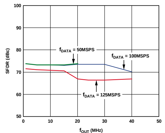
Figure 14. AD9779A Out-of-Band SFDR vs. f_{OUT} , 8 \times Interpolation
