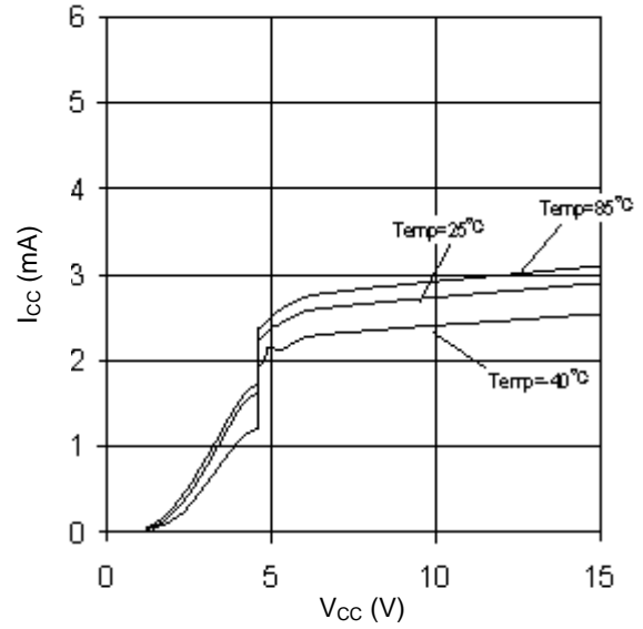
Figure 5. Circuit Current vs V_{CC}
