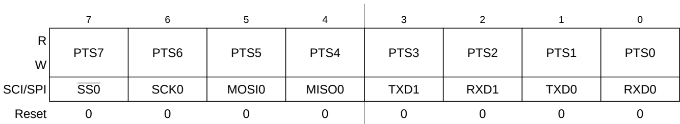
Figure 24-21. Port S Data Register (PTS)
