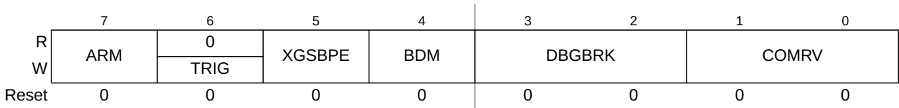
Figure 20-3. Debug Control Register (DBG1)
