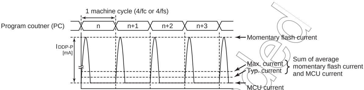
Figure 22-1 Intermittent Operation of Flash Memory
