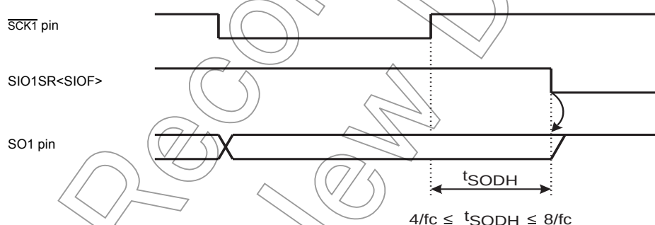
Figure 14-8 Hold Time of the End of Transmit Mode
