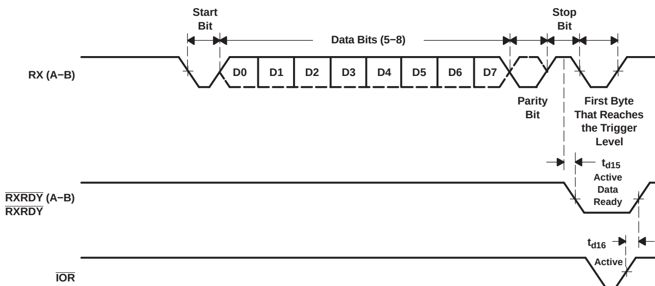
Figure 17. Receive Timing in FIFO Mode
