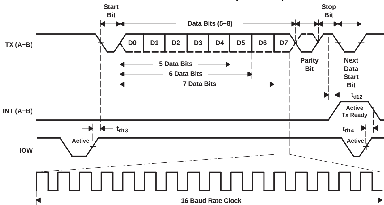
Figure 18. Transmit Timing
