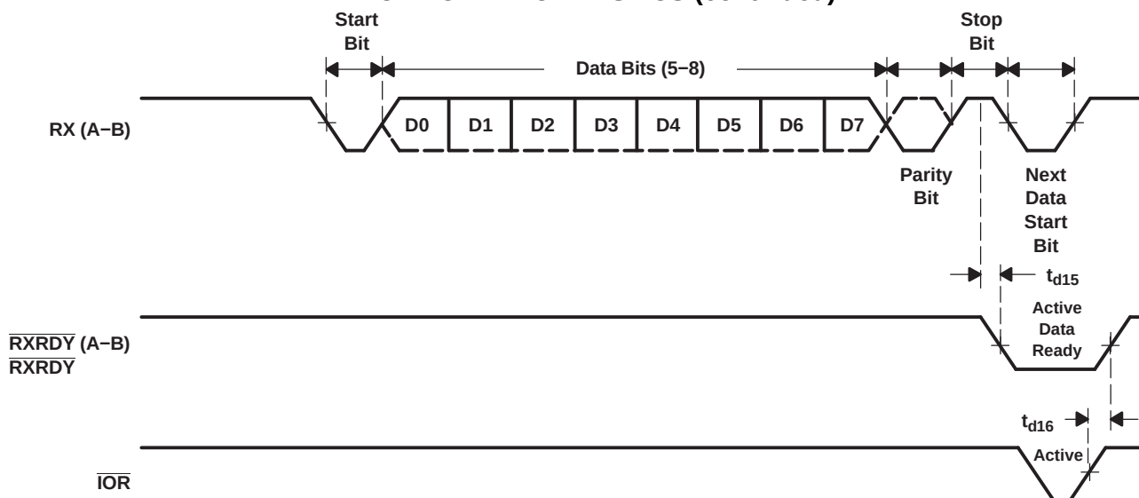
Figure 16. Receive Ready Timing in Non-FIFO Mode
