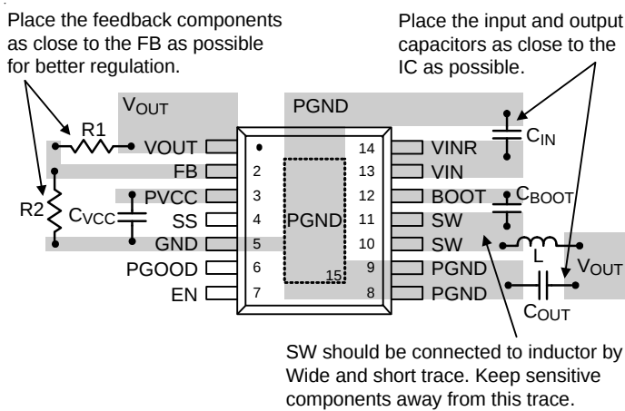
(a). For TSSOP-14 (Exposed Pad) Package
