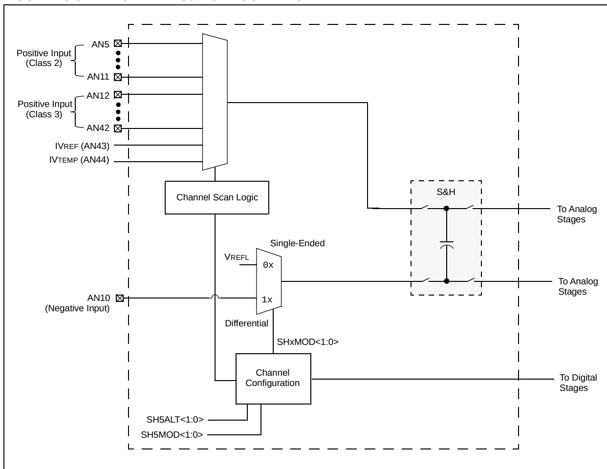
FIGURE 28-3: SHARED S&H 5 BLOCK DIAGRAM
