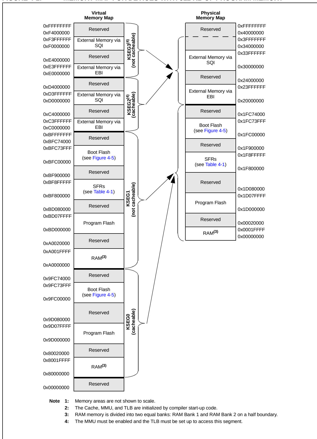
FIGURE 4-1: MEMORY MAP FOR DEVICES WITH 512 KB OF PROGRAM MEMORY (1,2)
