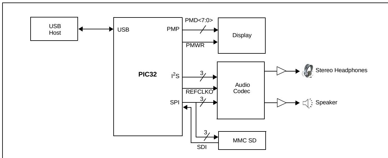
FIGURE 2-9: AUDIO PLAYBACK APPLICATION
