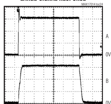
OPERATIONAL AMPLIFIER LARGE-SIGNAL RESPONSE
