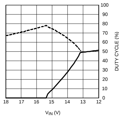
Figure 10. Mode Dependence on Duty Cycle (V OUT =12 V)
