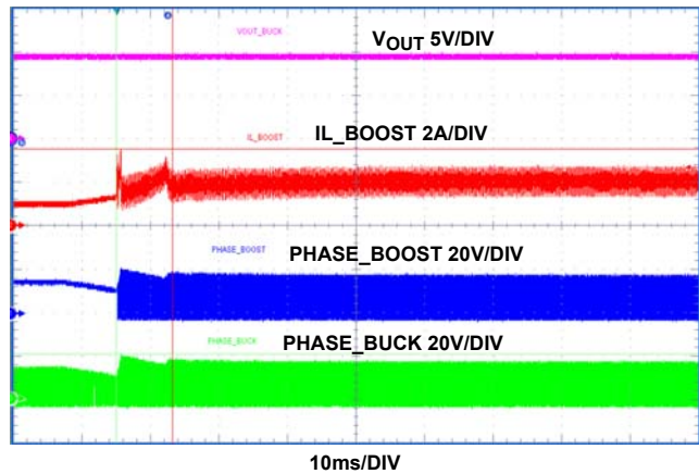
FIGURE 26. BOOST BUCK MODE, V_0 = 9V , I_0 = 1.8A , BOOST INPUT DROPS FROM 16V TO 9V DC
