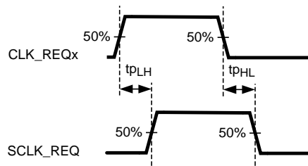
Figure 2. Clock Request Timing Waveforms
