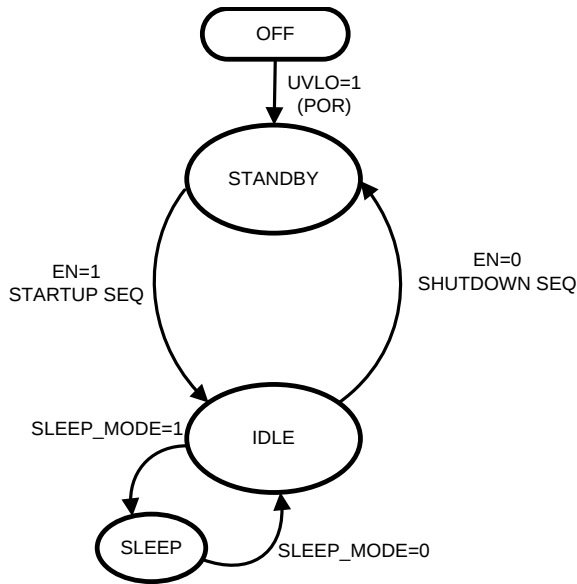
Figure 1. SUB-PMU Mode, CONFIG = 0
