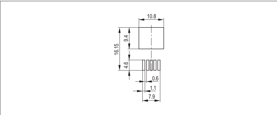
Figure 8 Foot Print for P-TO263-5-1 (Plastic Transistor Single Outline)
