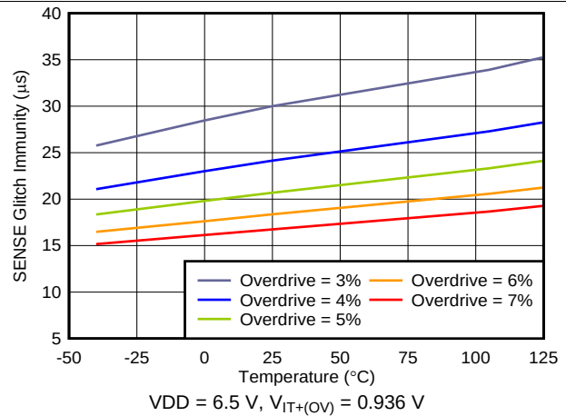
Figure 19. SENSE Glitch Immunity vs Temperature
