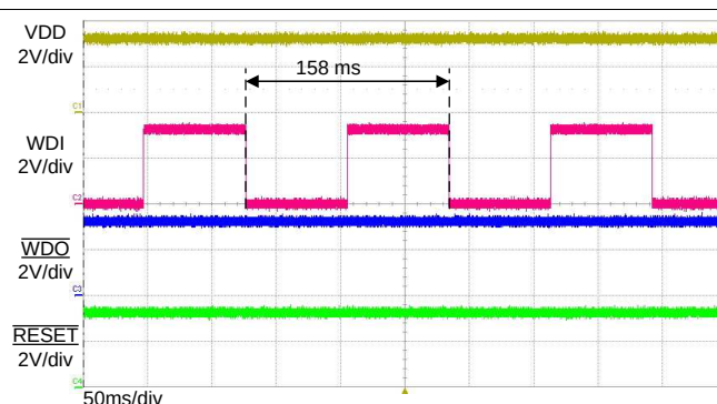
Figure 41. Typical WDI Signal
