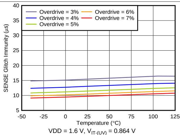
Figure 20. SENSE Glitch Immunity vs Temperature
