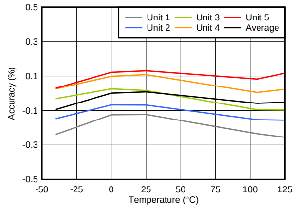
Figure 5. V_{IT-(UV)} Accuracy vs Temperature
