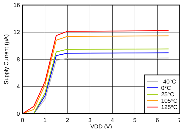
Figure 11. Supply Current vs Power-Supply Voltage
