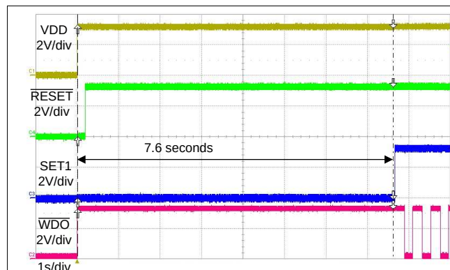
Figure 40. Startup Without a WDI Signal
