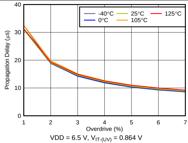
Figure 17. Propagation Delay vs Overdrive
