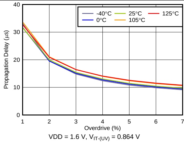
Figure 16. Propagation Delay vs Overdrive
