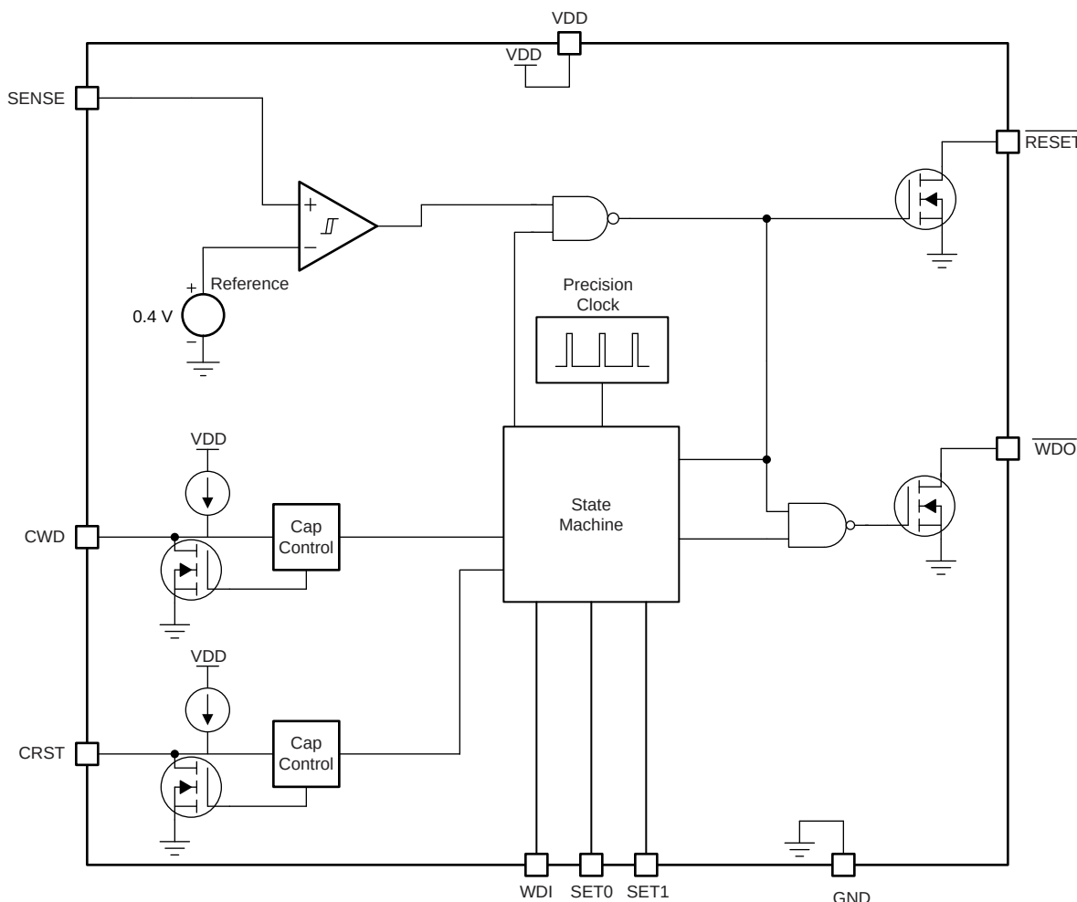
Figure 22. Adjustable Version Block Diagram
