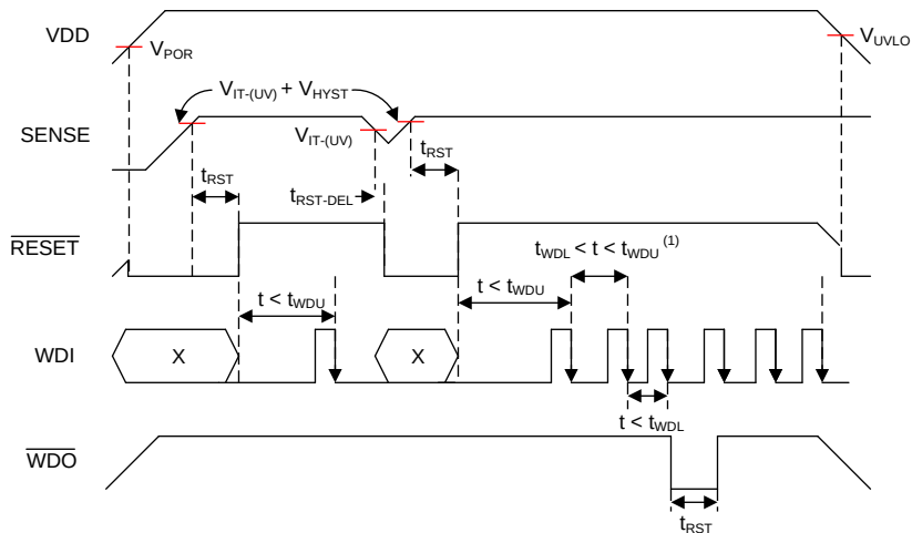
Figure 1. Timing Diagram
