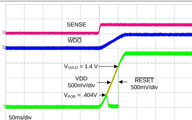
Figure 34. Startup Waveform
