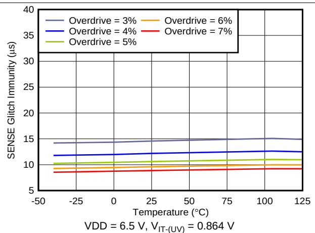
Figure 21. SENSE Glitch Immunity vs Temperature
