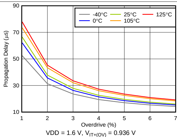
Figure 14. Propagation Delay vs Overdrive
