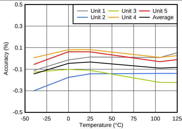
Figure 4. V_{IT+(OV)} Accuracy vs Temperature
