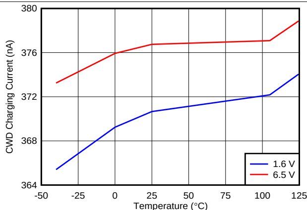
Figure 10. CWD Charging Current vs Temperature
