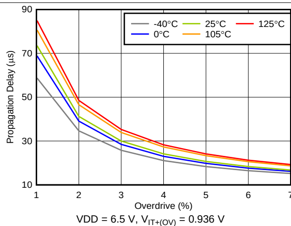
Figure 15. Propagation Delay vs Overdrive
