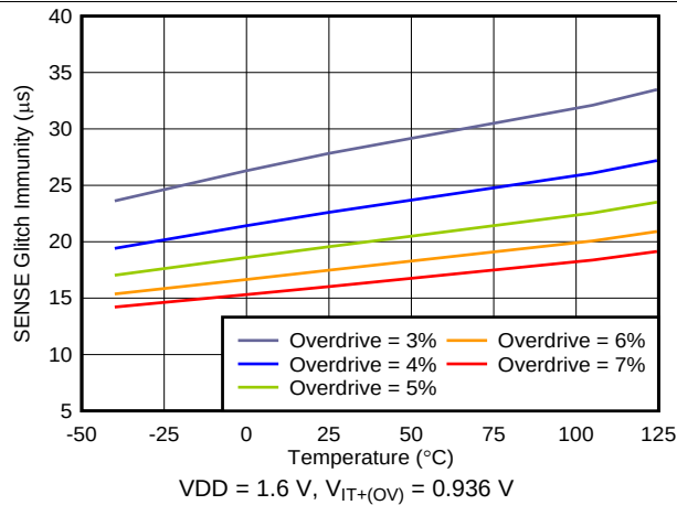
Figure 18. SENSE Glitch Immunity vs Temperature
