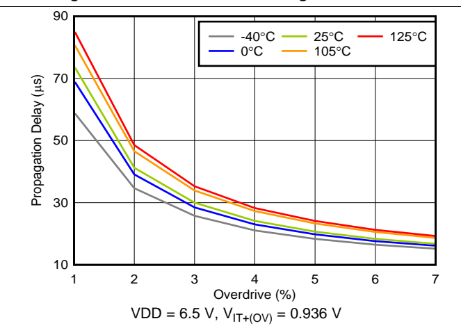
Figure 15. Propagation Delay vs Overdrive
