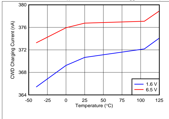
Figure 10. CWD Charging Current vs Temperature
