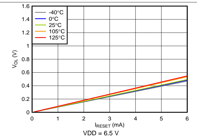
Figure 13. Low-Level \overline{\text{RESET}} Voltage vs \overline{\text{RESET}} Current
