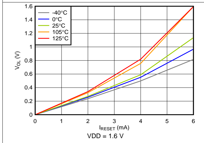
Figure 12. Low-Level \overline{\text{RESET}} Voltage vs \overline{\text{RESET}} Current
