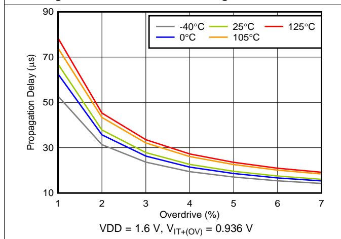
Figure 14. Propagation Delay vs Overdrive
