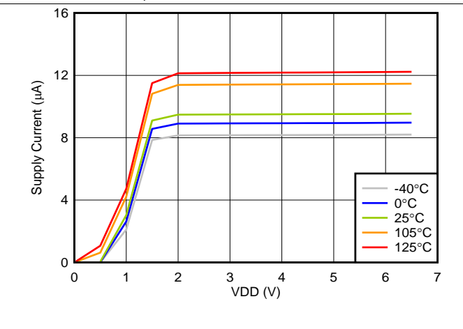
Figure 11. Supply Current vs Power-Supply Voltage
