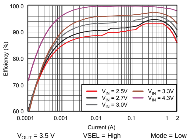
Figure 51. TPS61282A Efficiency vs Output Current
