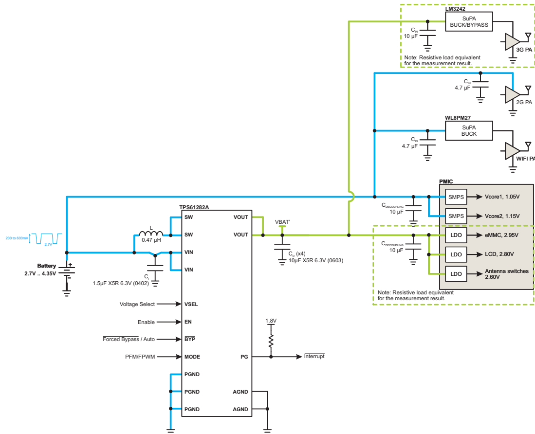
Figure 48. TPS61282A Application Circuit with 2000 mA Output Current
