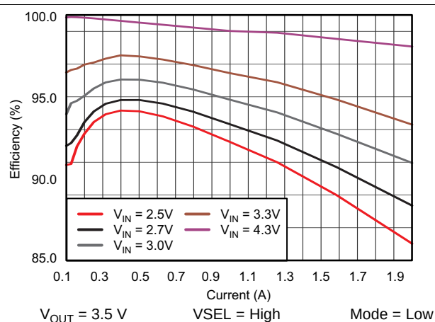
Figure 52. TPS61282A Efficiency vs Output Current
