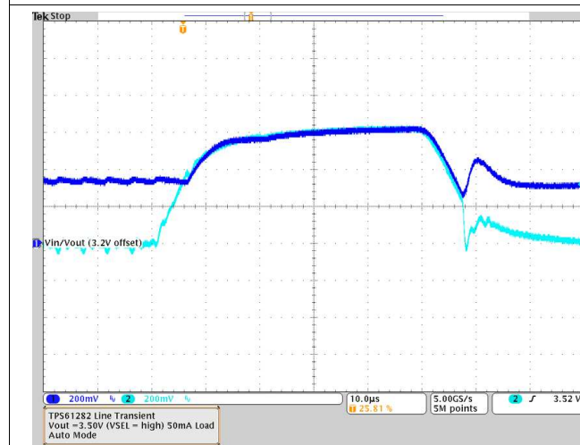
Figure 43. TPS61281A Forced Pass-Through to Boost Mode Transition
