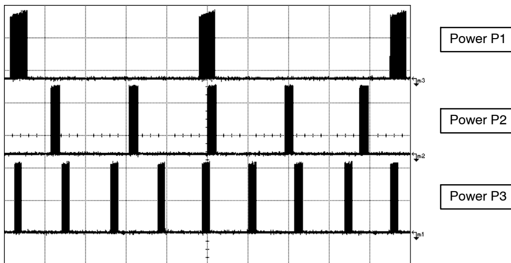
Figure 17. Output Pulses at Various Power Levels (X = 5.0 μs/div) P1 < P2 < P3
