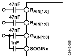
Figure 6. Typical Clamp Configuration for RGB/YUV Applications
