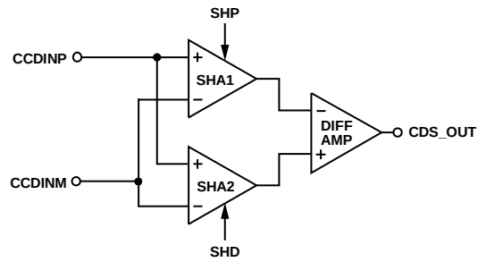
Figure 39. CDS Block Diagram (Conceptual)
