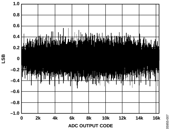
Figure 6. Differential Nonlinearity
