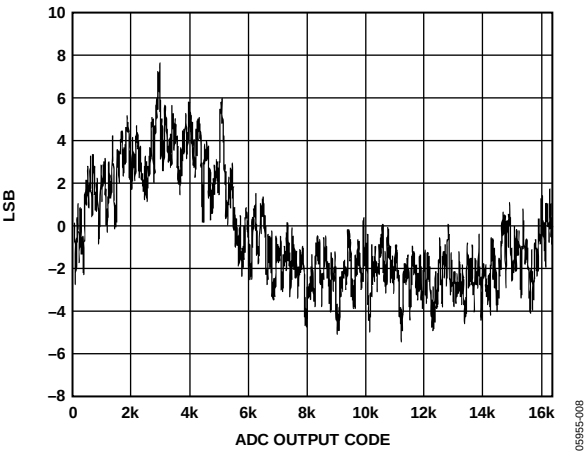
Figure 7. Integral Nonlinearity
