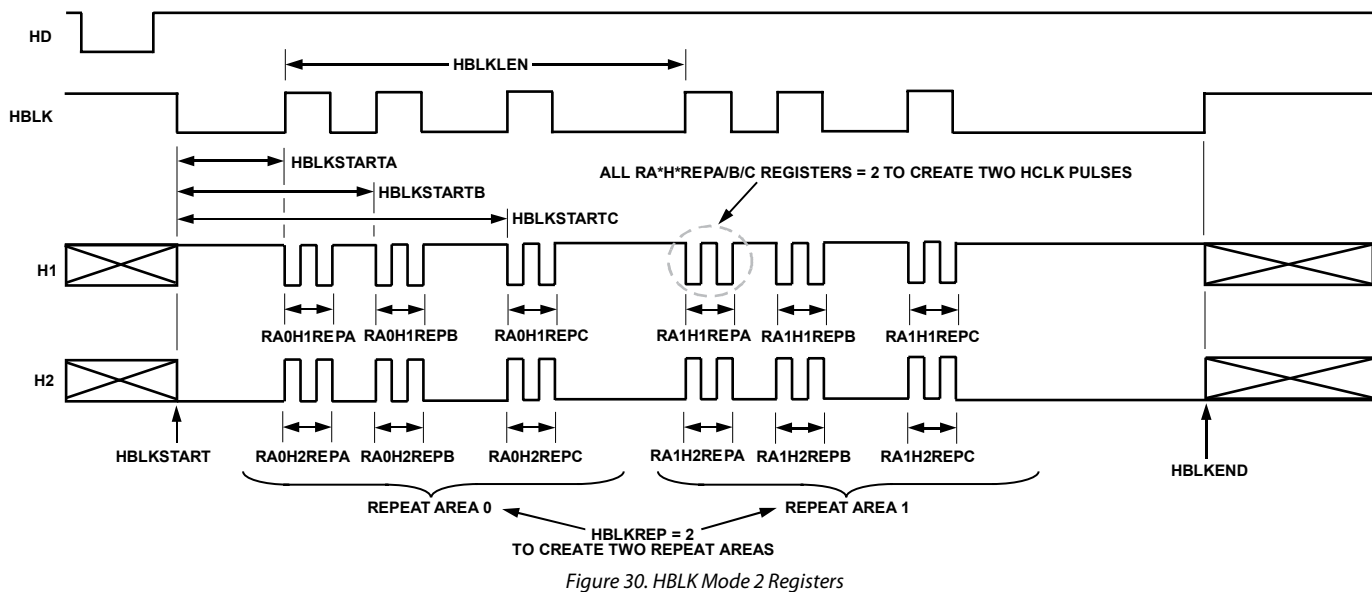
Figure 30. HBLK Mode 2 Registers
