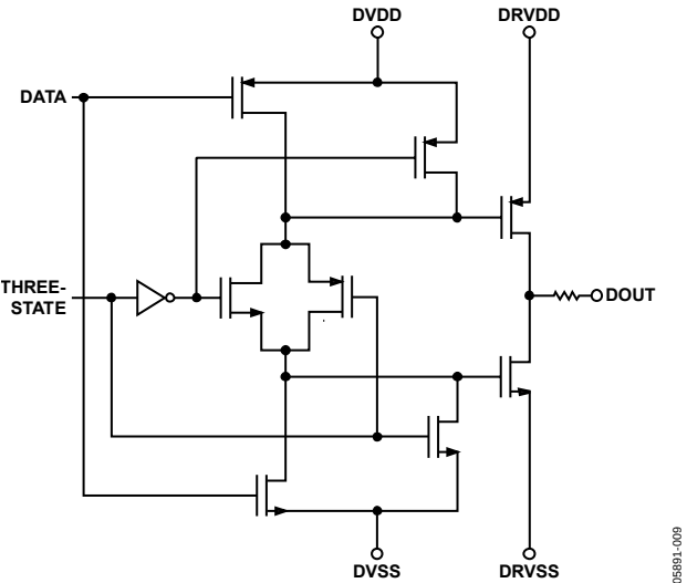
Figure 9. Digital Data Outputs
