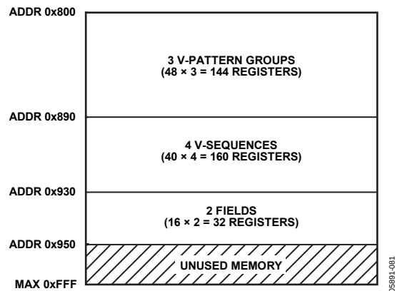
Figure 86. Example Register Configuration
