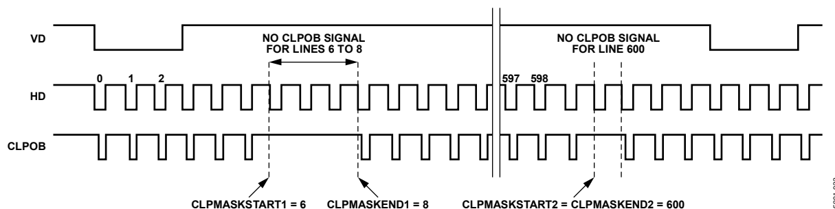
Figure 23. CLPOB Masking Example
