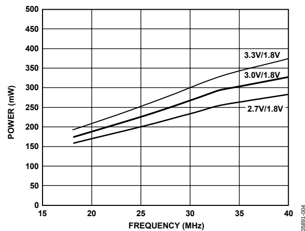
Figure 4. Power vs. Frequency (AVDD = TCVD = DVDD = 1.8 V, All Other Supplies at 2.7 V, 3.0 V, or 3.3 V)
