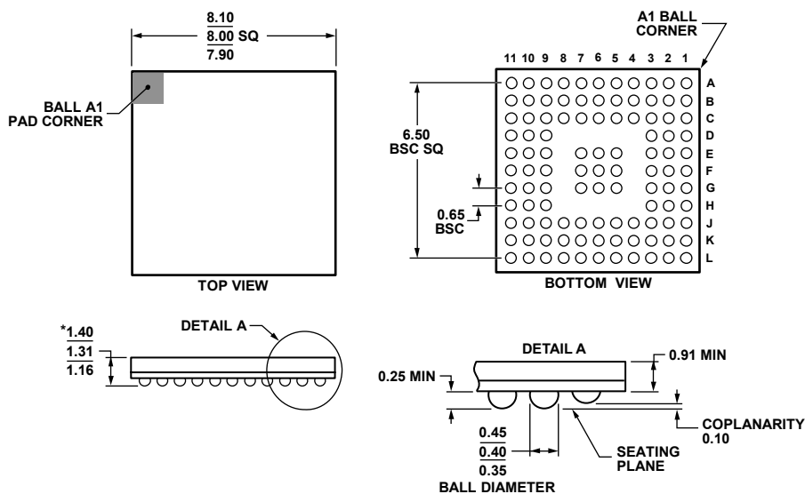
*COMPLIANT TO JEDEC STANDARDS MQ-225 WITH THE EXCEPTION TO PACKAGE HEIGHT. Figure 88. 105-Lead Chip Scale Package Ball Grid Array [CSP_BGA] 8 mm x 8 mm Body (BC-105-1) Dimensions shown in millimeters
