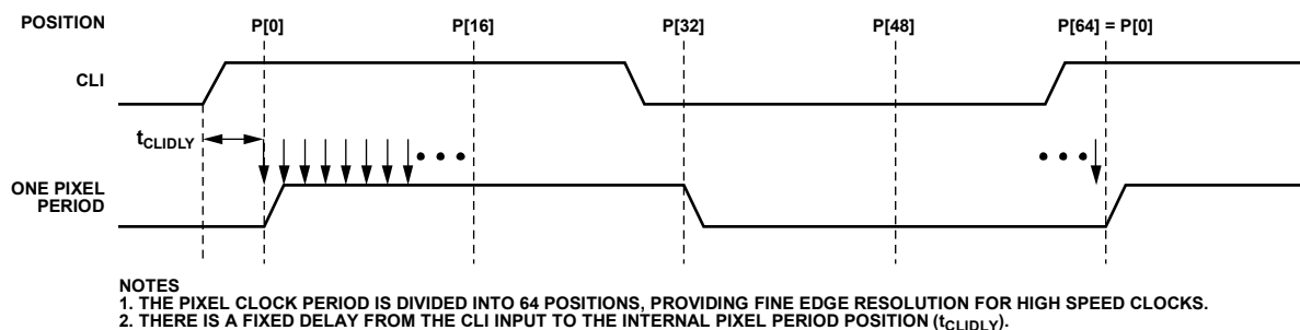
Figure 15. High Speed Clock Resolution from CLI, Master Clock Input
