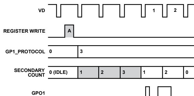
Figure 62. ShotDelay Toggle Operation Using GP1_PROTOCOL = 3
