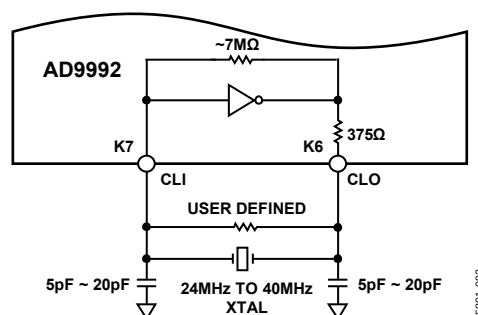
Figure 82. Crystal Application Using CLI/CLO (Consult Crystal Data Sheet for Component Values)
