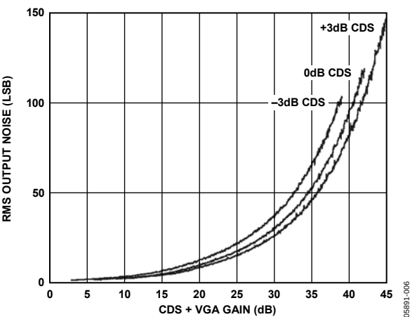
Figure 6. Output Noise vs. Total Gain (CDS + VGA)
