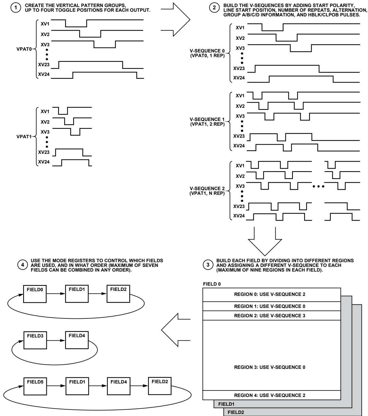
Figure 33. Summary of Vertical Timing Generation
