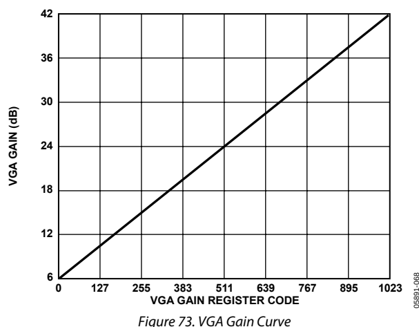
Figure 73. VGA Gain Curve
