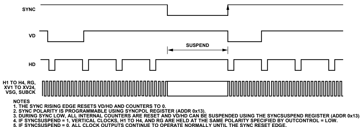
Figure 75. SYNC Timing to Synchronize the AD9992 with External Timing
