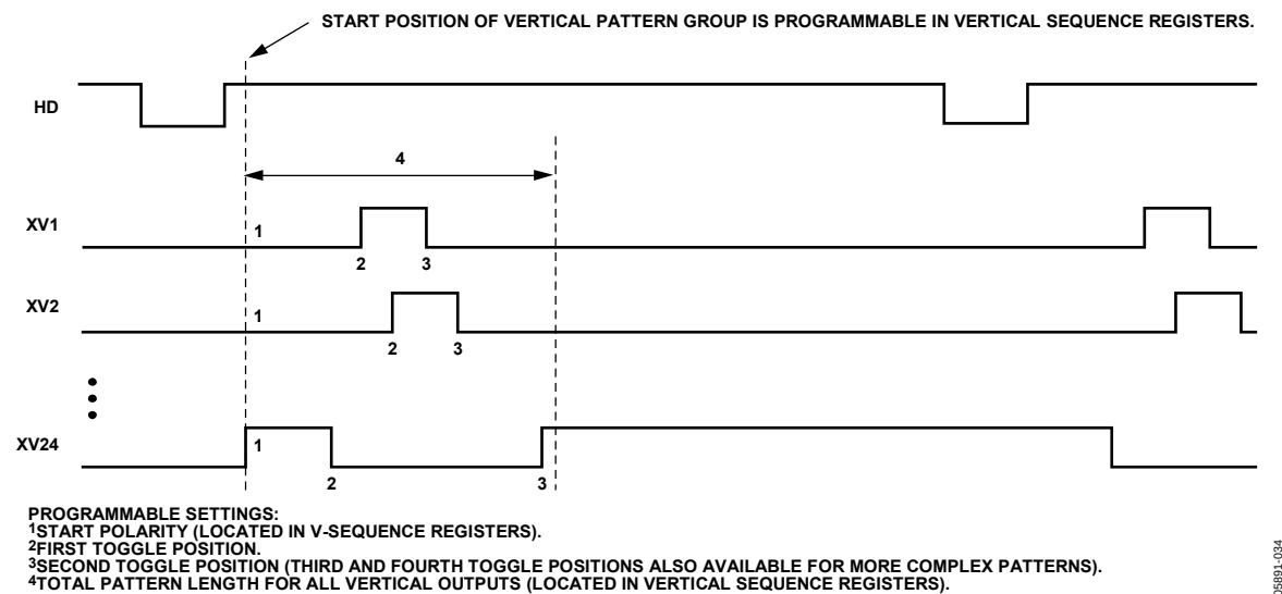
Figure 34. Vertical Pattern Group Programmability
