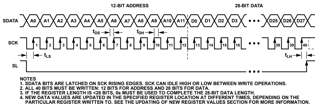
Figure 83. Serial Write Operation
