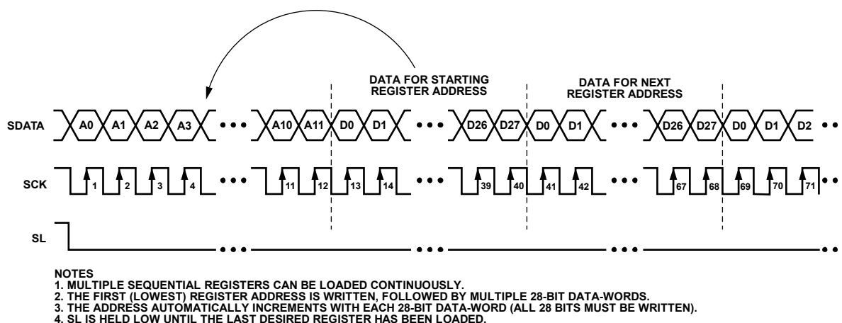
Figure 84. Continuous Serial Write Operation
