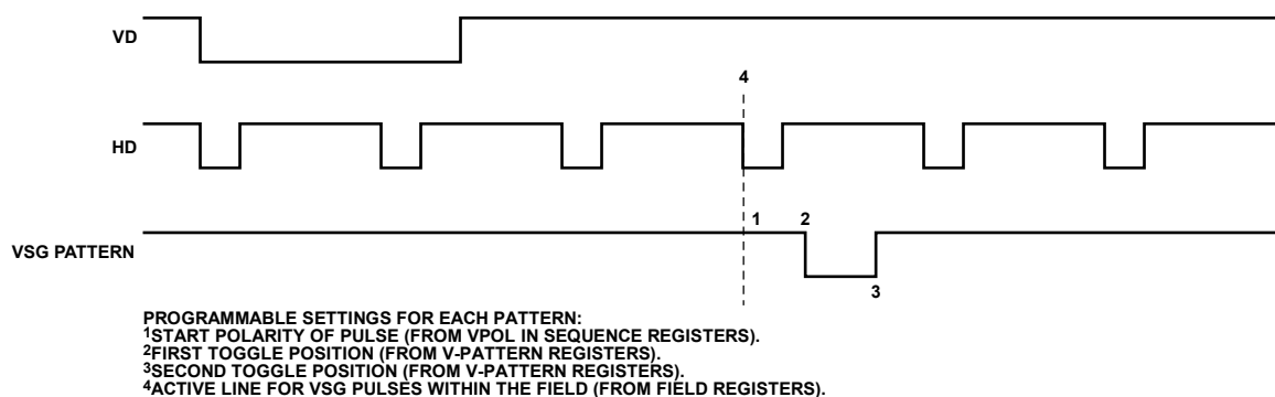
Figure 51. Vertical Sensor Gate Pulse Placement
