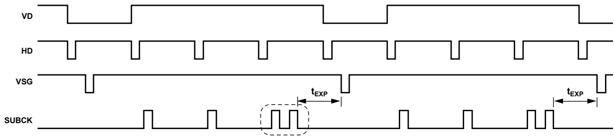
Figure 57. High Precision SUBCK Operation
