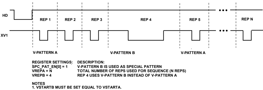
Figure 47. Example of Special Pattern Insertion, Detail
