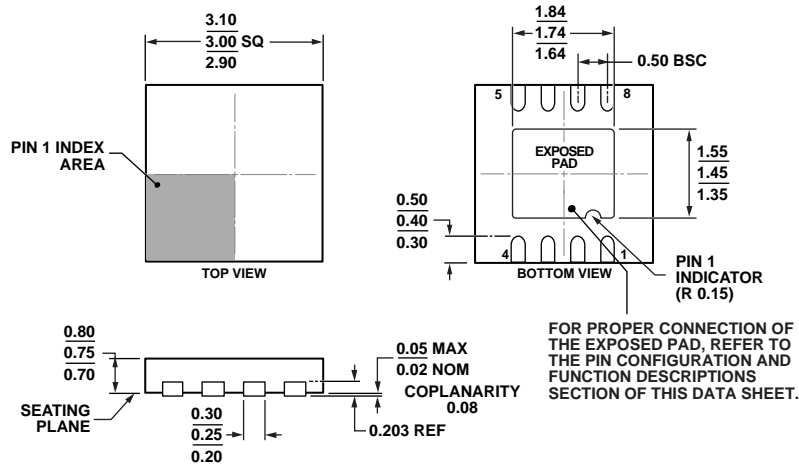
Figure 52. 8-Lead Lead Frame Chip Scale Package [LFCSP_WD] 3 mm x 3 mm Body, Very Very Thin, Dual Lead (CP-8-13)
