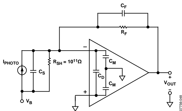
Figure 63. Wideband Photodiode Preamplifier
