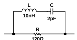
Figure 61. RLC Circuit
