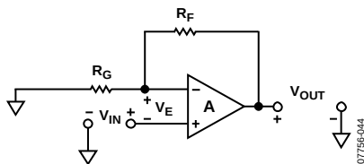
Figure 52. Noninverting Configuration
