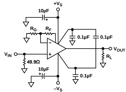
Figure 49. Noninverting Gain Configuration
