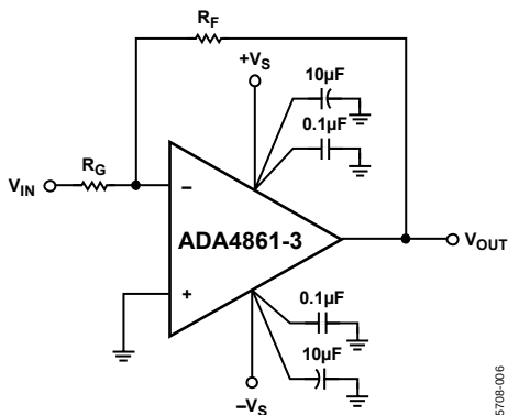
Figure 47. Inverting Gain
