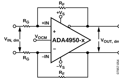
Figure 54. ADA4950-x Configured for Balanced (Differential) Inputs
