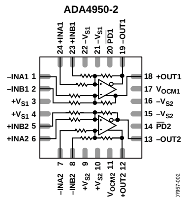
Figure 2. ADA4950-2
