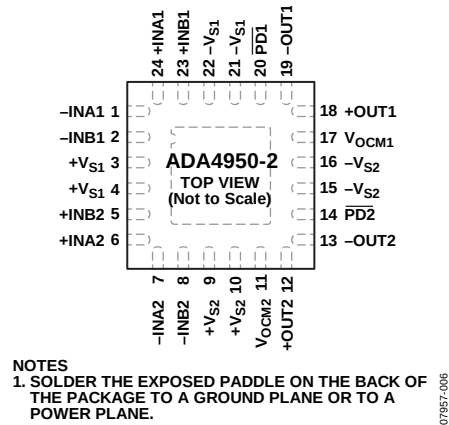
Figure 6. ADA4950-2 Pin Configuration
