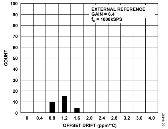
Figure 16. Offset Drift, External Reference, PGIA Gain = 6.4
