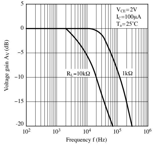
Fig.14 Frequency Response
