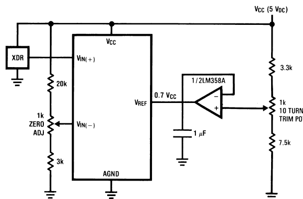
Figure 13. Operating with Ratiometric Transducers
