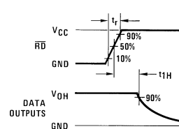
Figure 16. t_{1H} , C_L=10 pF
