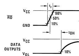
Figure 18. t_{0H} , C_L=10 pF
