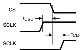
Figure 5. SCLK and CS Timing Parameters
