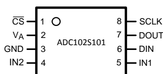
Figure 1. 8-Lead VSSOP See DGK Package
