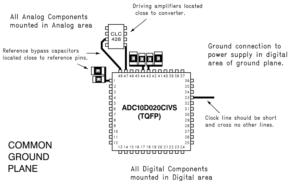
Figure 68. An Acceptable Layout Pattern
