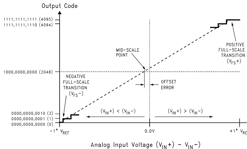
Figure 4. Transfer Characteristic
