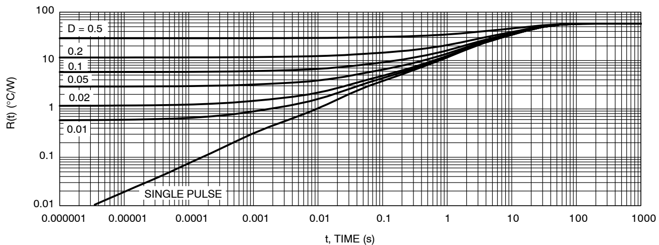
Figure 13. Thermal Response
