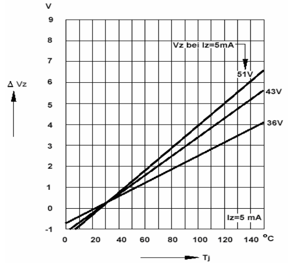
Fig 14. Change of Zener Voltage vs Tj
