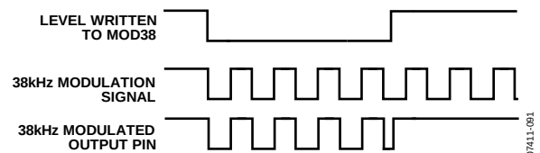
Figure 119. 38 kHz Modulation
