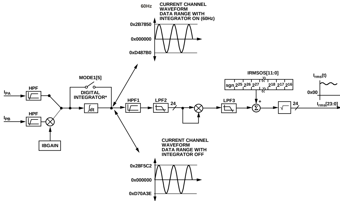
Figure 61. ADE5166/ADE5169 Current Channel RMS Signal Processing with PGA1 = 2, 4, 8, or 16
