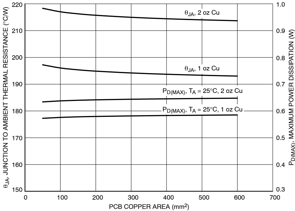
Figure 54. \theta_{JA} and P_{D(MAX)} vs. Copper Area (XDFN4)
