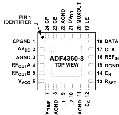
Figure 3. Pin Configuration
