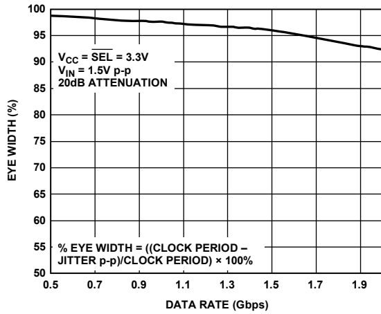
Figure 22. Eye Width vs. Data Rate; PRBS 31
