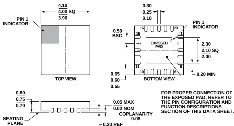
Figure 12. 20-Lead Lead Frame Chip Scale Package [LF CSP_WQ] 4 mm × 4 mm Body, Very Very Thin Quad (CP-20-6)
