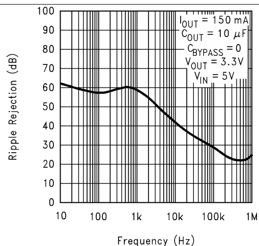
Figure 6. Ripple Rejection
