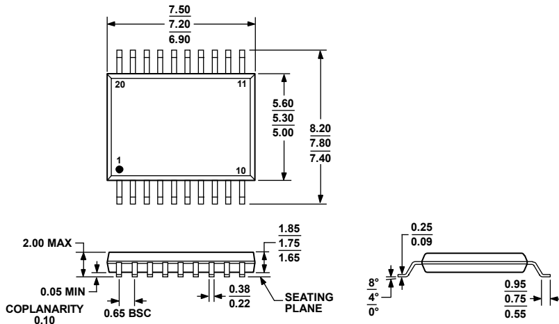
Figure 25. 20-Lead Shrink Small Outline Package [SSOP] (RS-20)
