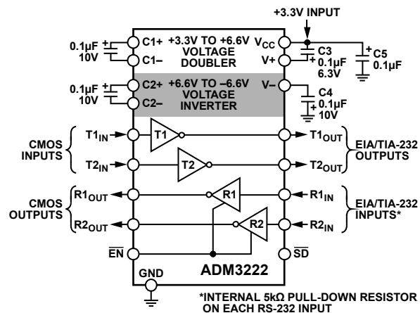
Figure 16. ADM3222 Typical Operating Circuit
