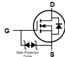
Equivalent Circuit
