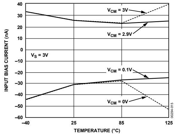
Figure 10. Input Bias Current vs. Temperature, V_S = 3\text{ V}
