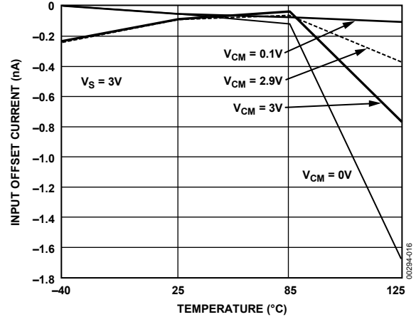
Figure 11. Input Offset Current vs. Temperature, V_S = 3\text{ V}
