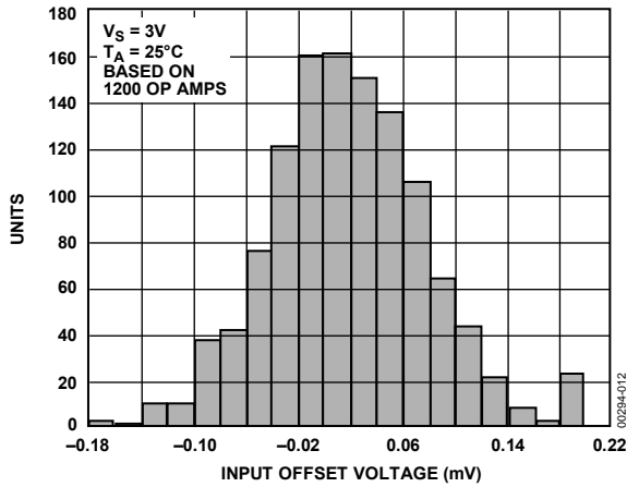
Figure 7. OP291 Input Offset Voltage Distribution, V_S = 3\text{ V}
