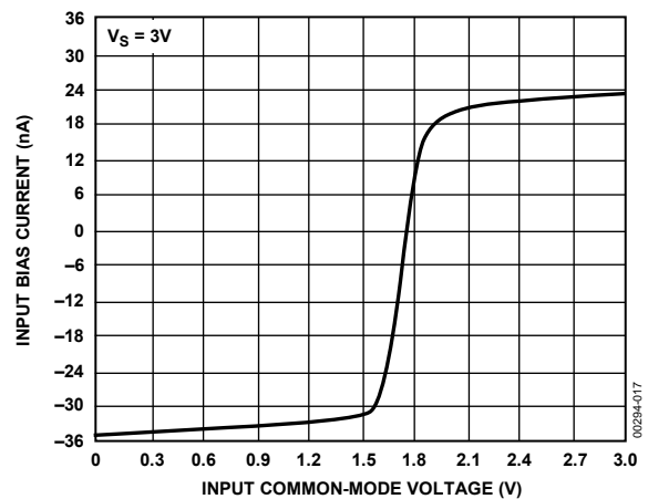
Figure 12. Input Bias Current vs. Input Common-Mode Voltage, V_S = 3\text{ V}
