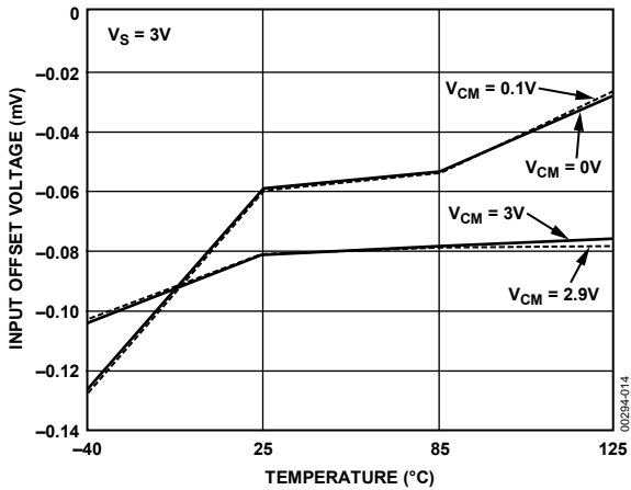
Figure 9. Input Offset Voltage vs. Temperature, V_S = 3\text{ V}
