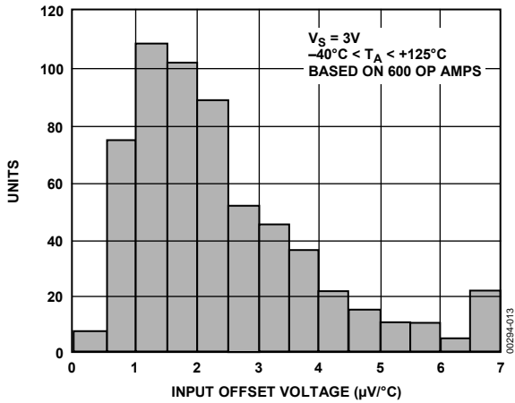
Figure 8. OP291 Input Offset Voltage Drift Distribution, V_S = 3\text{ V}
