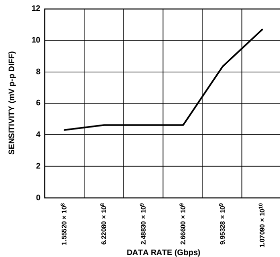
Figure 17. Sensivities of SONET/SDH Data Rates (BER = 10 -10 )
