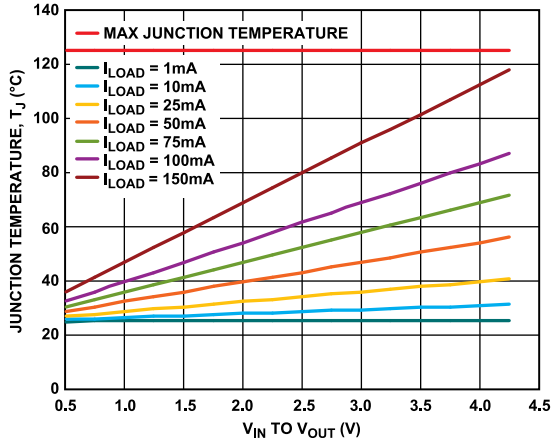
Figure 34. TSOT, 100 mm 2 of PCB Copper, T A = 25°C
