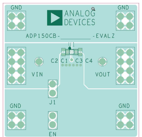
Figure 48. Example WLCSP PCB Layout
