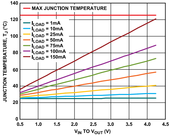
Figure 40. WLCSP, 500 mm 2 of PCB Copper, T_A = 25^\circ\text{C}
