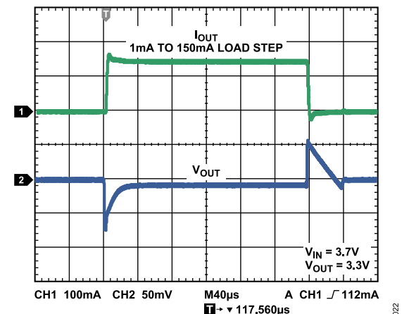
Figure 22. Load Transient Response, C_{OUT} = 1\text{ }\mu\text{F}
