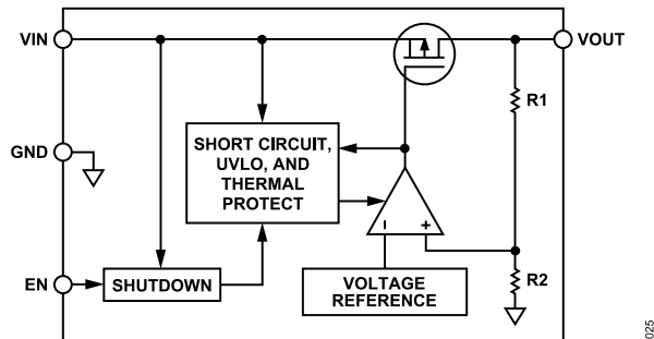
Figure 26. Internal Block Diagram
