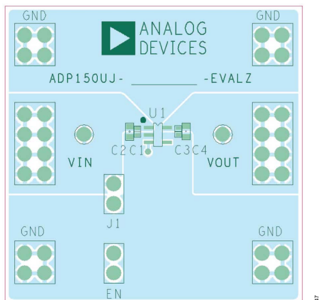
Figure 47. Example TSOT PCB Layout
