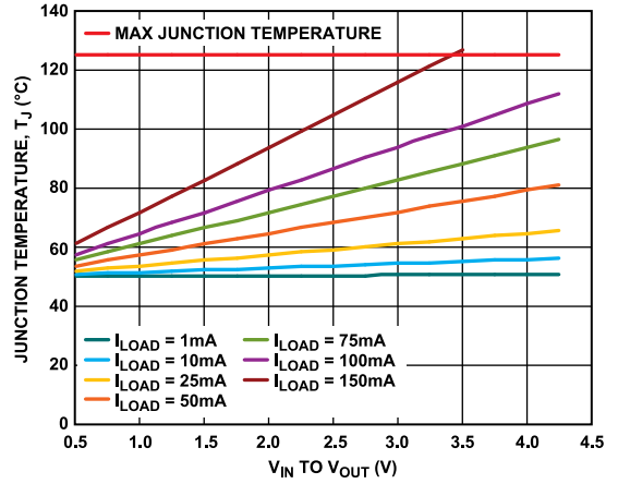
Figure 37. TSOT, 100 mm 2 of PCB Copper, T A = 50°C
