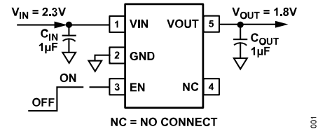
Figure 1. 5-Lead TSOT with Fixed Output Voltage, 1.8 V
