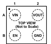
Figure 4. 4-Ball WLCSP Pin Configuration
