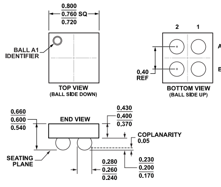
Figure 50. 4-Ball Wafer Level Chip Scale Package [WLCSP] (CB-4-3) Dimensions shown in millimeters
