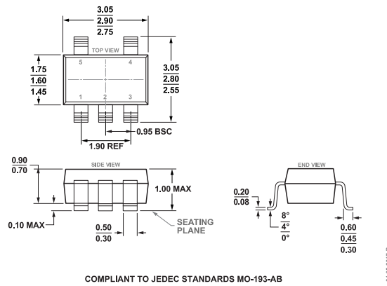
Figure 49. 5-Lead Thin Small Outline Transistor Package [TSOT] (UJ-5) Dimensions shown in millimeters
