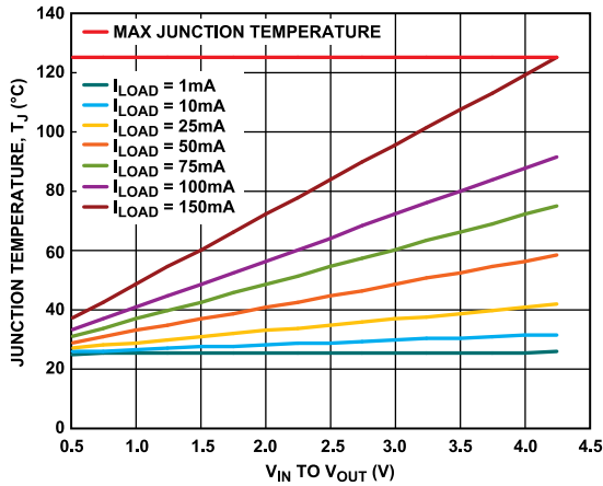
Figure 41. WLCSP, 100 mm 2 of PCB Copper, T_A = 25^\circ\text{C}
