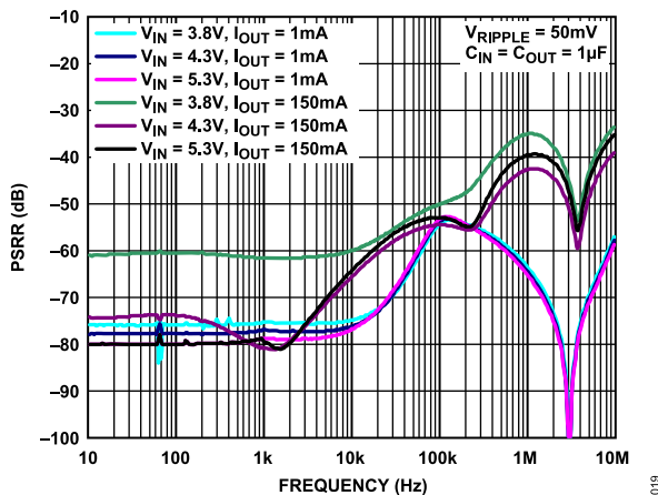
Figure 19. Power Supply Rejection Ratio (PSRR) vs. Frequency with Various Headroom Voltages ( V_{IN} - V_{OUT} ), V_{OUT} = 3.3\text{ V}
