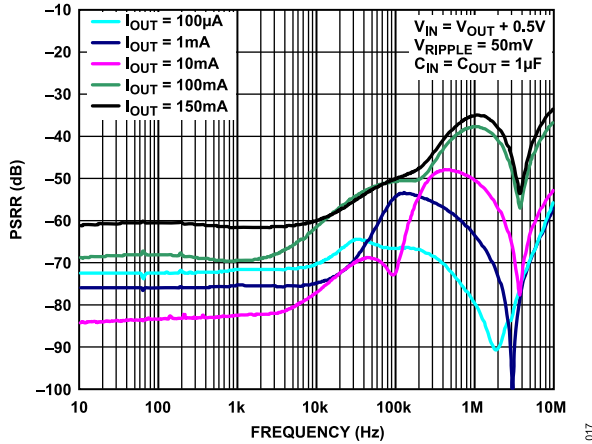
Figure 17. Power Supply Rejection Ratio (PSRR) vs. Frequency, V_{OUT} = 3.3\text{ V} , V_{IN} = 3.8\text{ V}
