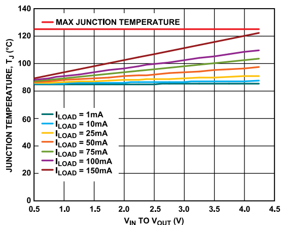
Figure 46. WLCSP, 100 mm 2 of PCB Copper, Board Temperature = 85°C
