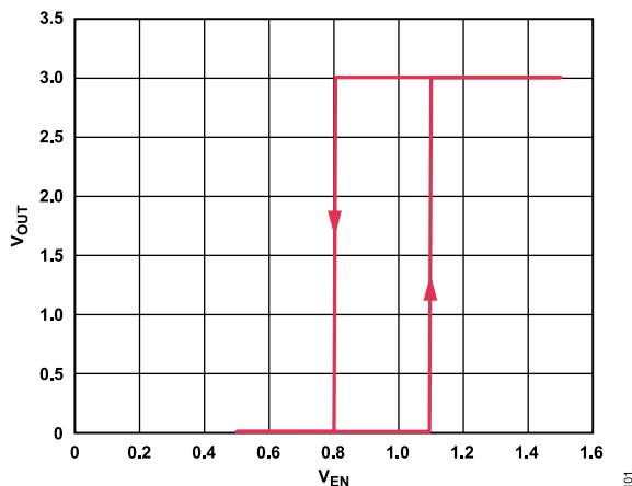
Figure 30. Typical EN Pin Operation
