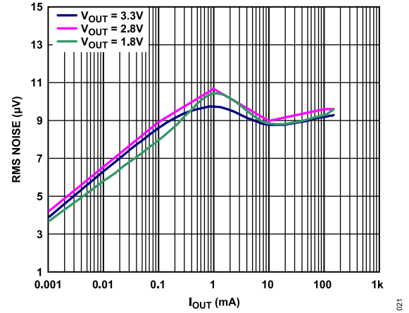
Figure 20. Output RMS Noise vs. Load Current ( I_{OUT} ) and Output Voltage ( V_{OUT} ), V_{IN} = 5\text{ V} , C_{OUT} = 1\text{ }\mu\text{F}
