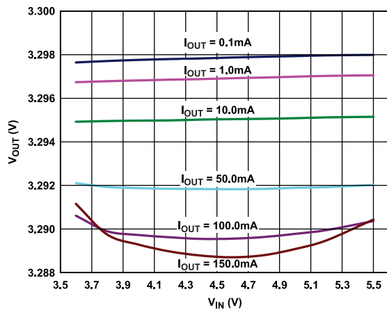
Figure 7. Output Voltage ( V_{OUT} ) vs. Input Voltage ( V_{IN} )
