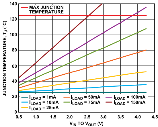
Figure 42. WLCSP, 0 mm 2 of PCB Copper, T_A = 25^\circ\text{C}
