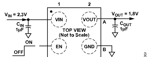
Figure 2. 4-Ball WLCSP with Fixed Output Voltage, 1.8 V
