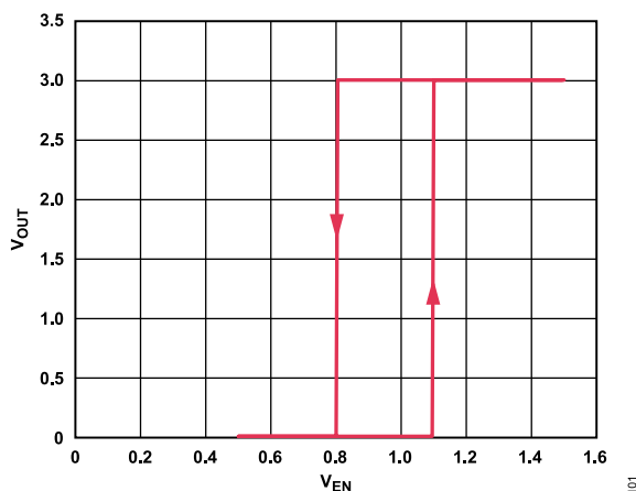
Figure 30. Typical EN Pin Operation
