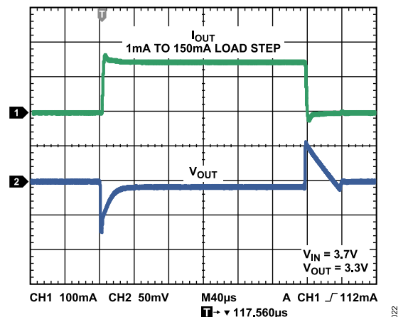
Figure 22. Load Transient Response, C_{OUT} = 1\text{ }\mu\text{F}
