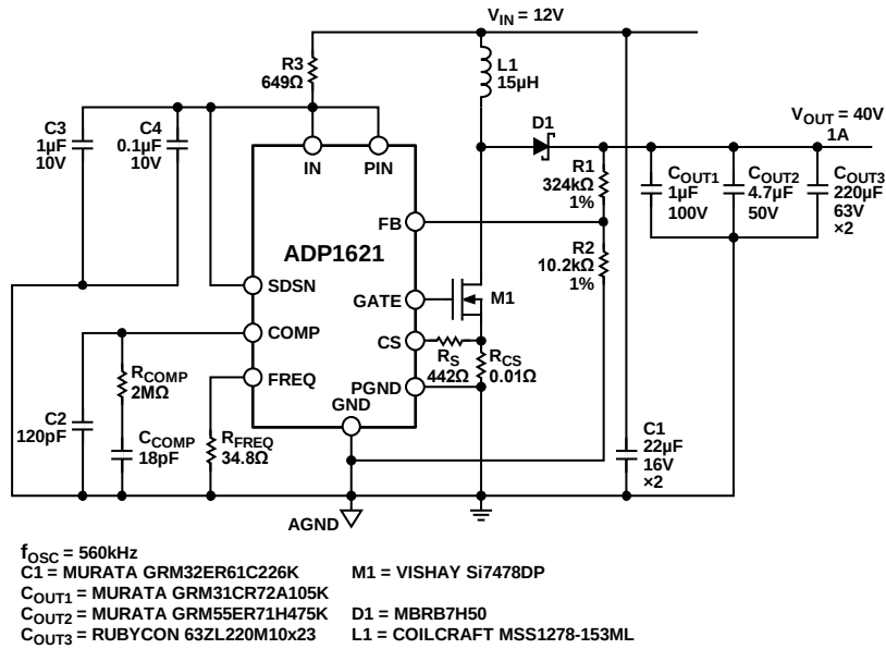
Figure 38. High Input Voltage and High Output Voltage Converter
