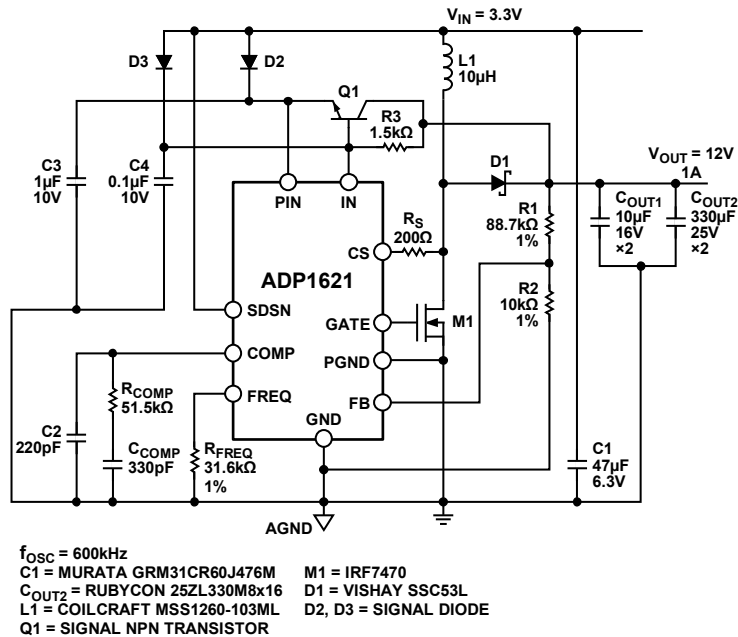
Figure 35. Bootstrapped Application Circuit for V_{OUT} > 5.5\text{ V}
