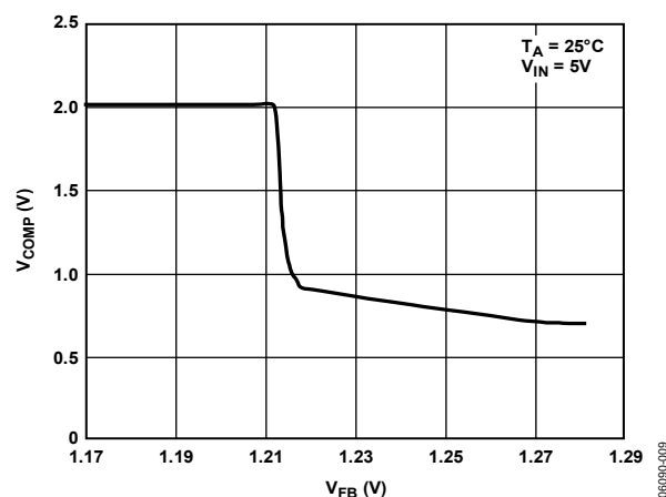
Figure 10. V_{\text{COMP}} vs. V_{\text{FB}}
