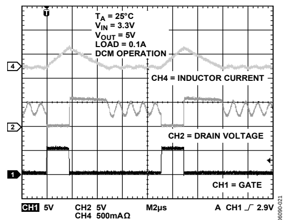
Figure 22. DCM Switching Waveform
