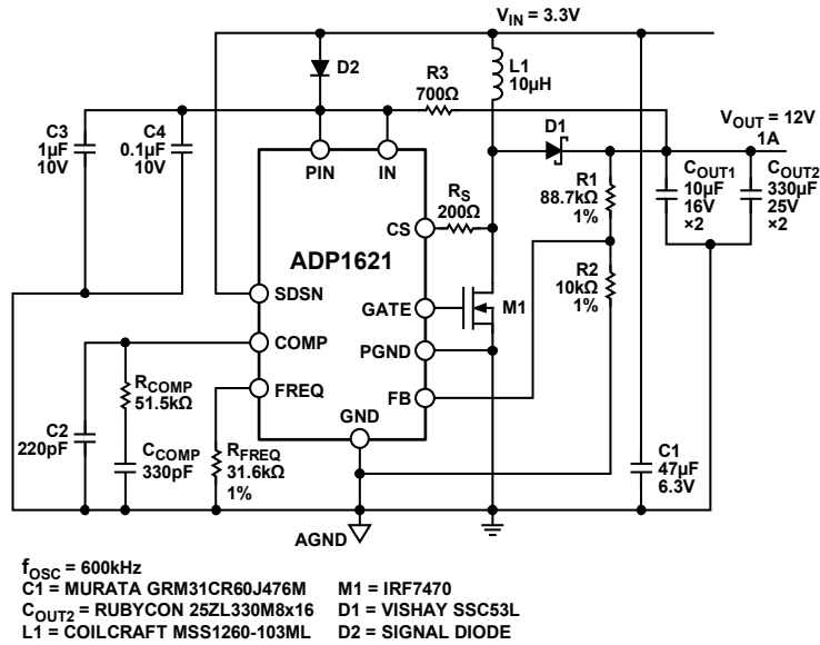
Figure 34. Bootstrapped Application Circuit for V_{OUT} > 5.5\text{ V}
