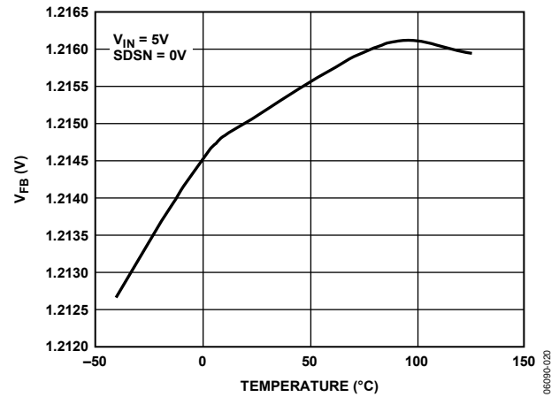
Figure 21. FB Voltage vs. Temperature
