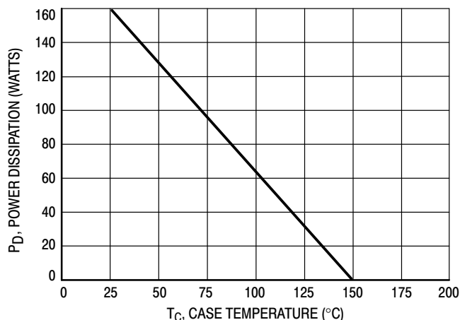
Figure 1. Power Derating
