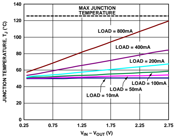
Figure 43. 500 mm 2 of PCB Copper, T_B = 50^\circ\text{C} , LFCSP
